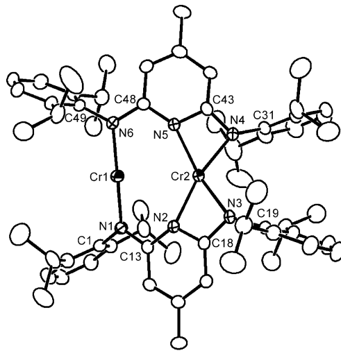
Figure 3. Molecular structure of the Cr-containing anion of 5 with thermal ellipsoids at 35% probability. The counter cation [(\text{Et}_2\text{O})\text{K}[\text{18}\text{crown-6}]]^+ , diethyl ether solvate, and hydrogen atoms have been omitted for clarity.
