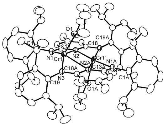
Figure 2. Molecular structure of 3 with thermal ellipsoids at 35% probability. Hydrogen atoms have been omitted for clarity.
